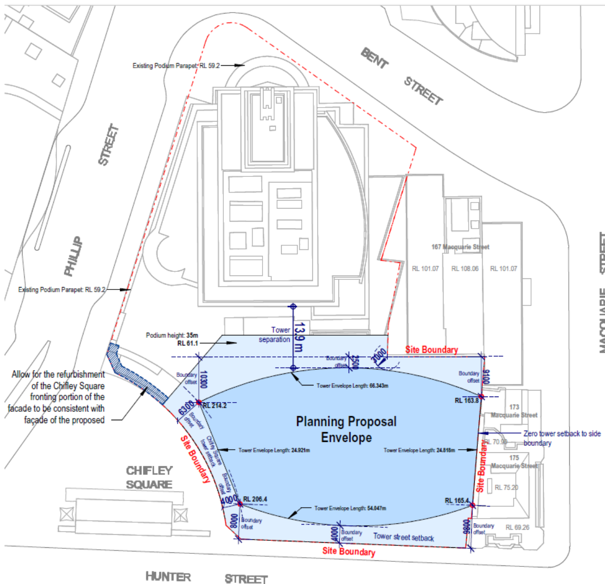
Figure 3 Extent of competitive design process in blue (southern podium and tower), plan view
